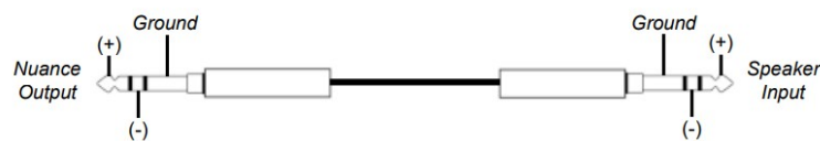
Fig. 1: Typical wiring between the Nuance Outputs and balanced inputs
