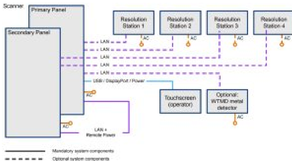
Figure 6-1: Connection overview
