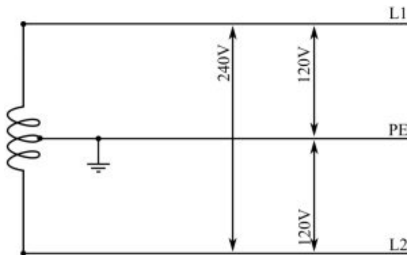
Single phase, 2 wire
