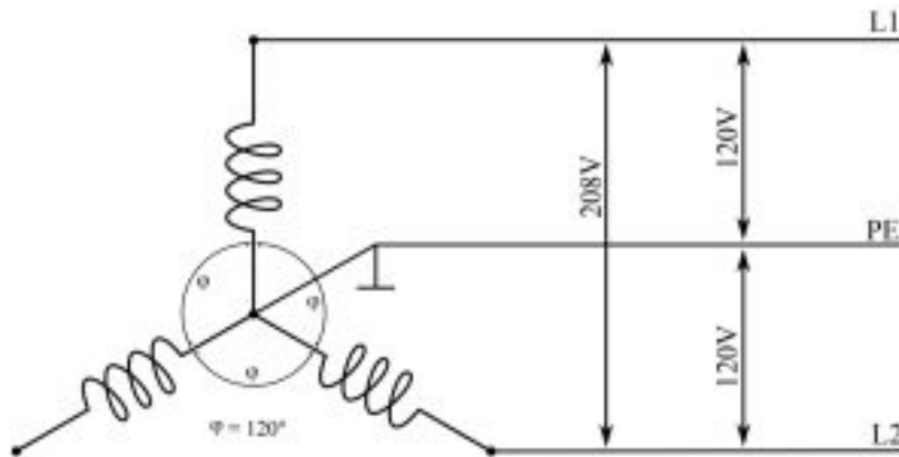
3-Phase Wye
