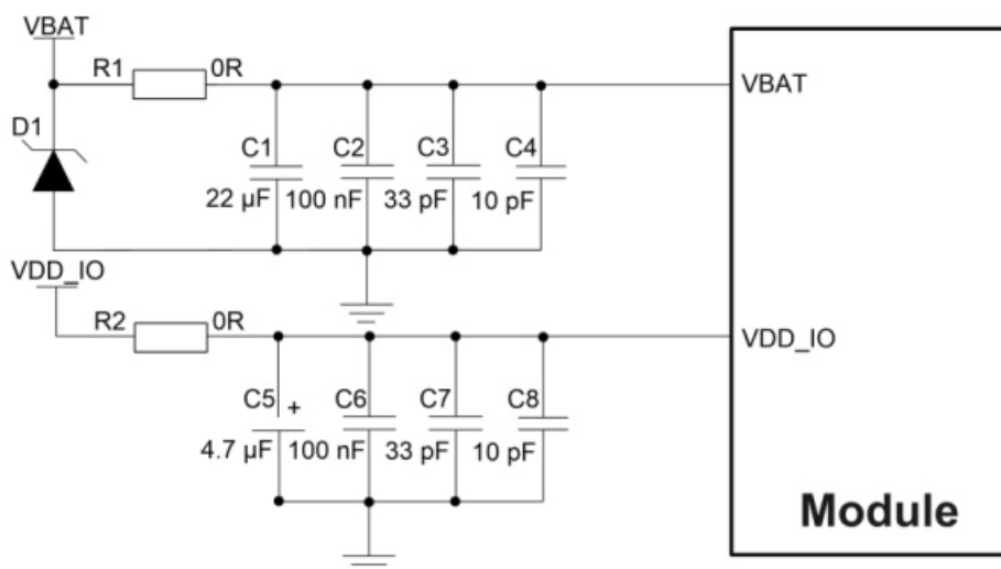
Figure 3: Reference Design for Power Supply
