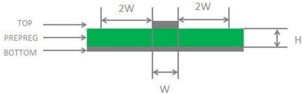
Figure 15: Microstrip Design on a 2-layer PCB
