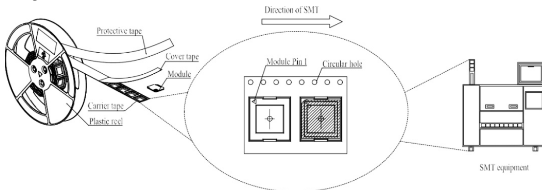
Figure 30: Mounting Direction
