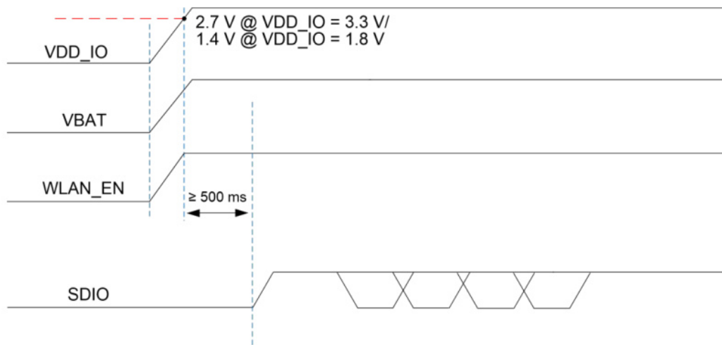
Figure 4: Power-up Timing
