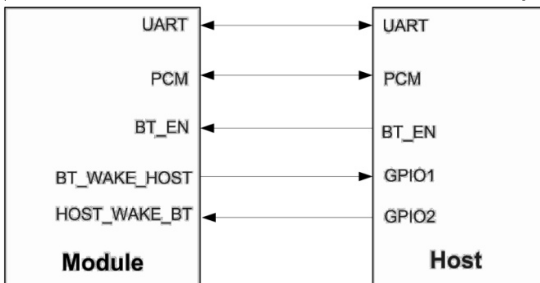
Figure 8: Bluetooth Application Interface Connection
