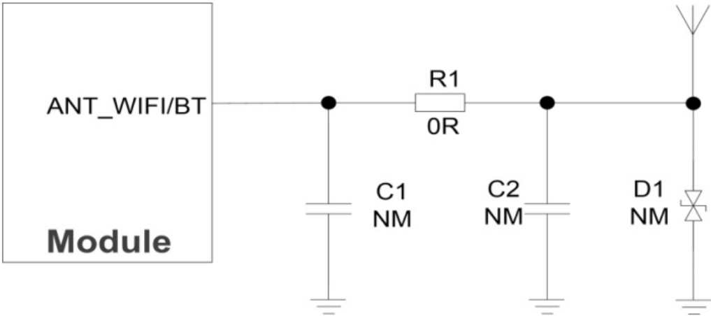
Figure 14: Reference Design of RF Antenna Interface
