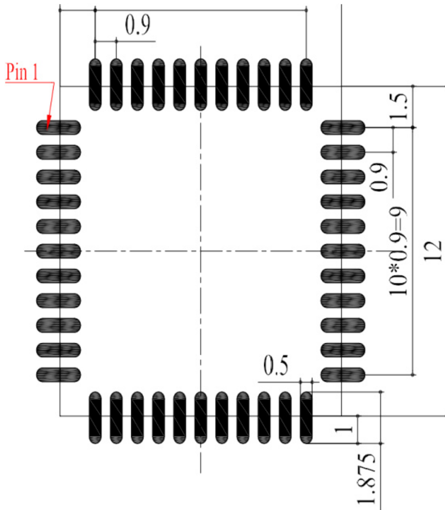
Figure 25: Recommended Footprint
