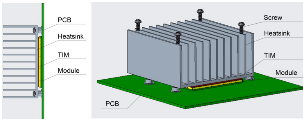
Figure 22: Placement and Fixing of the Heatsink
