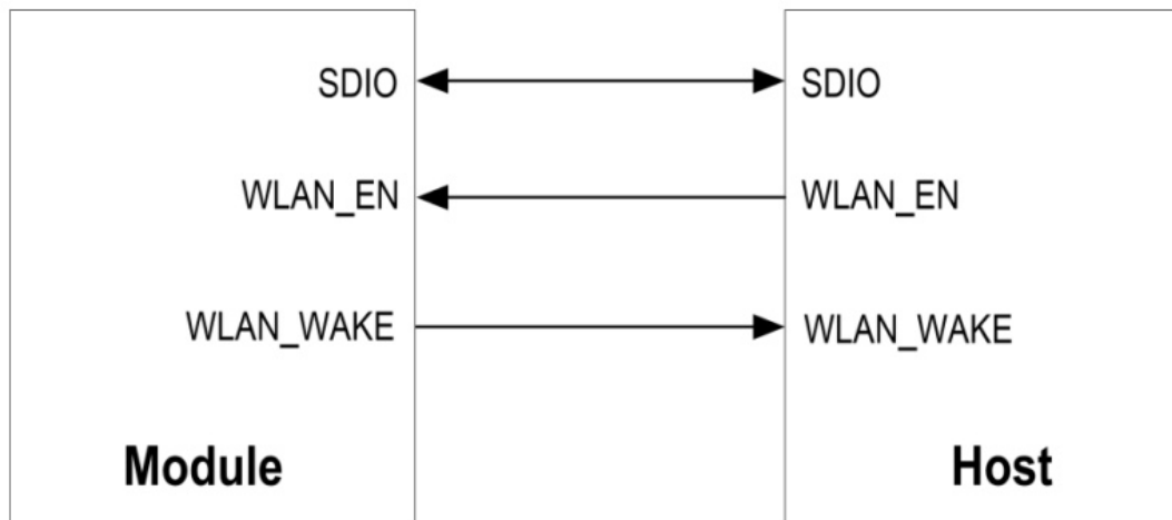
Figure 5: Wi-Fi Application Interface Connection
