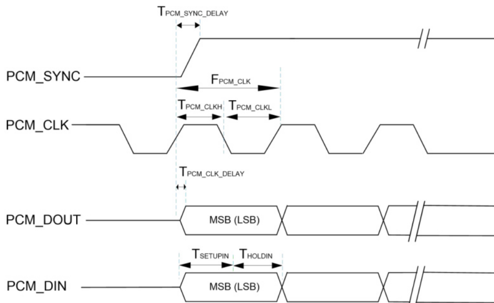
Figure 9: PCM interface Timing (Long Frame Sync)
