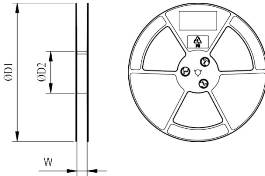
Figure 29: Plastic Reel Dimension Drawing
