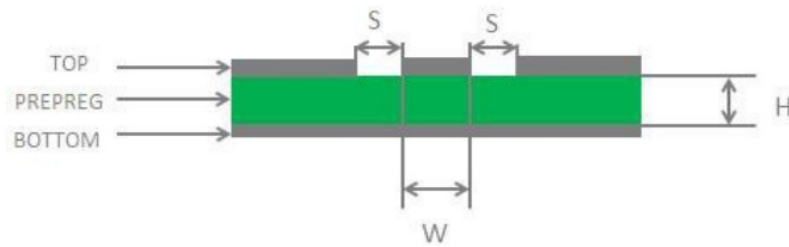
Figure 16: Coplanar Waveguide Design on a 2-layer PCB
