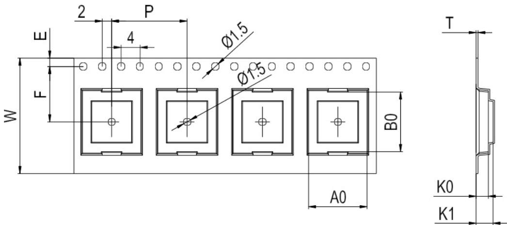
Figure 28: Carrier Tape Dimension Drawing
