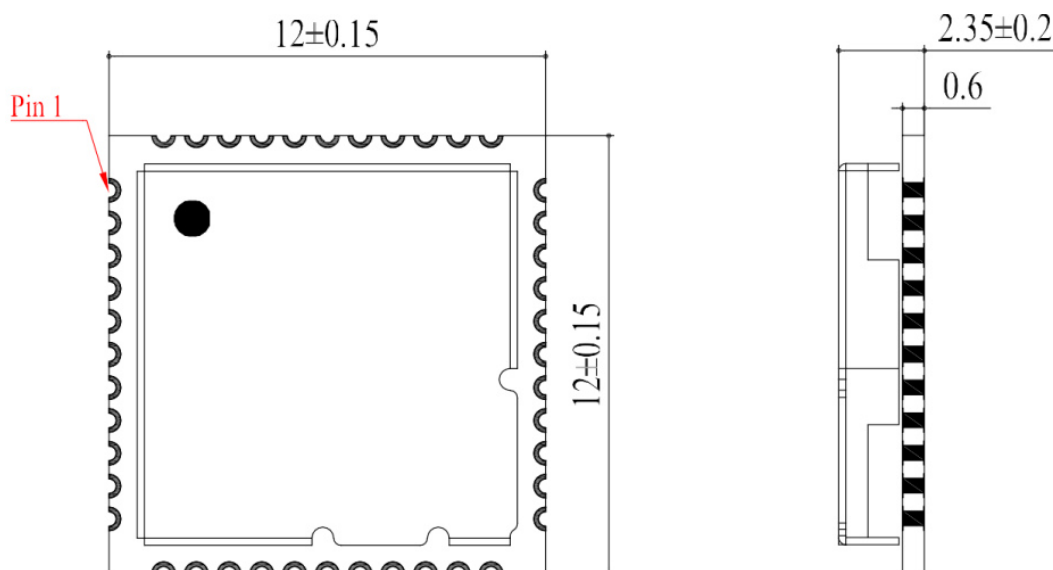
Figure 23: Top and Side Dimensions
