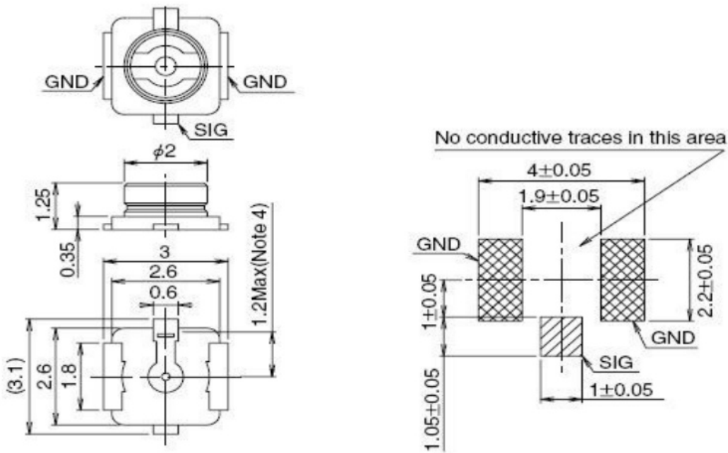
Figure 19: Dimensions of the Receptacle (Unit: mm)
