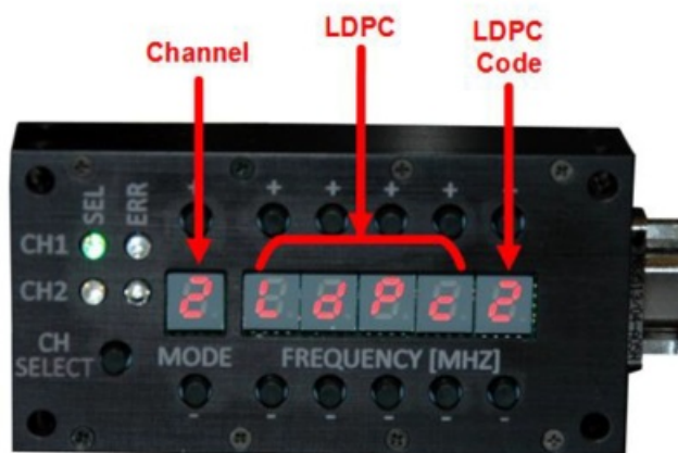
Figure 8: Labeled LDPC Display Example, Channel 2, LDPC Code 2
