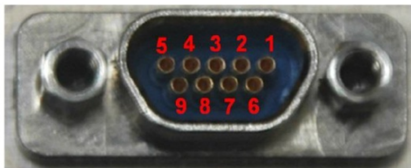
Figure 12: Female MDM-9 Connector
