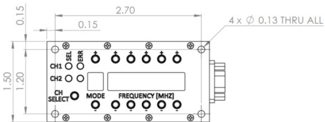
Figure 13: 2 nd Generation Switch Box Drawing
