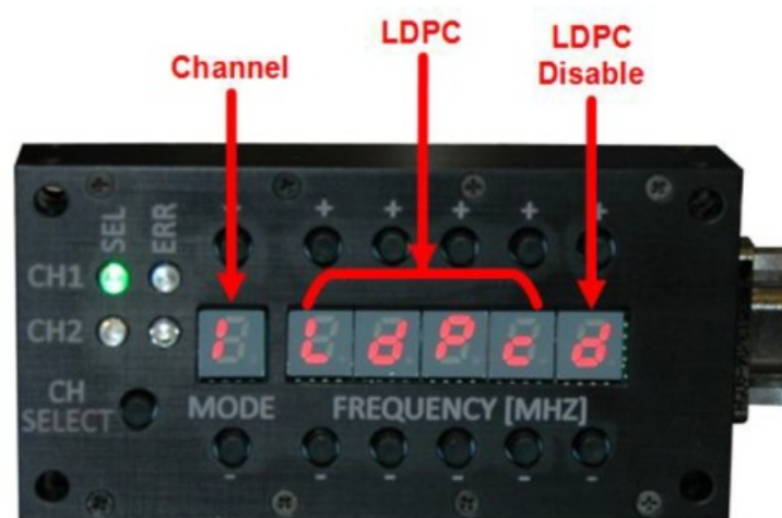
Figure 9: Labeled LDPC Display Example, LDPC Disabled
