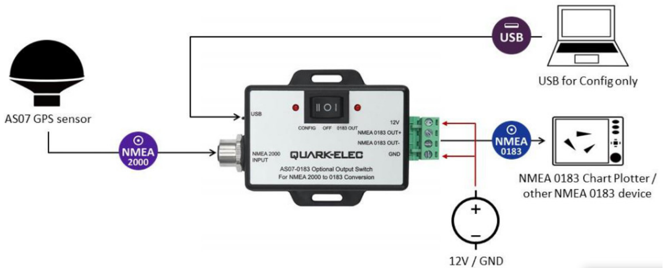
Figure 5: AS07-C Connections
