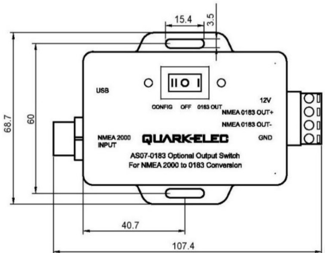
Figure 4 AS07-C Dimensions
