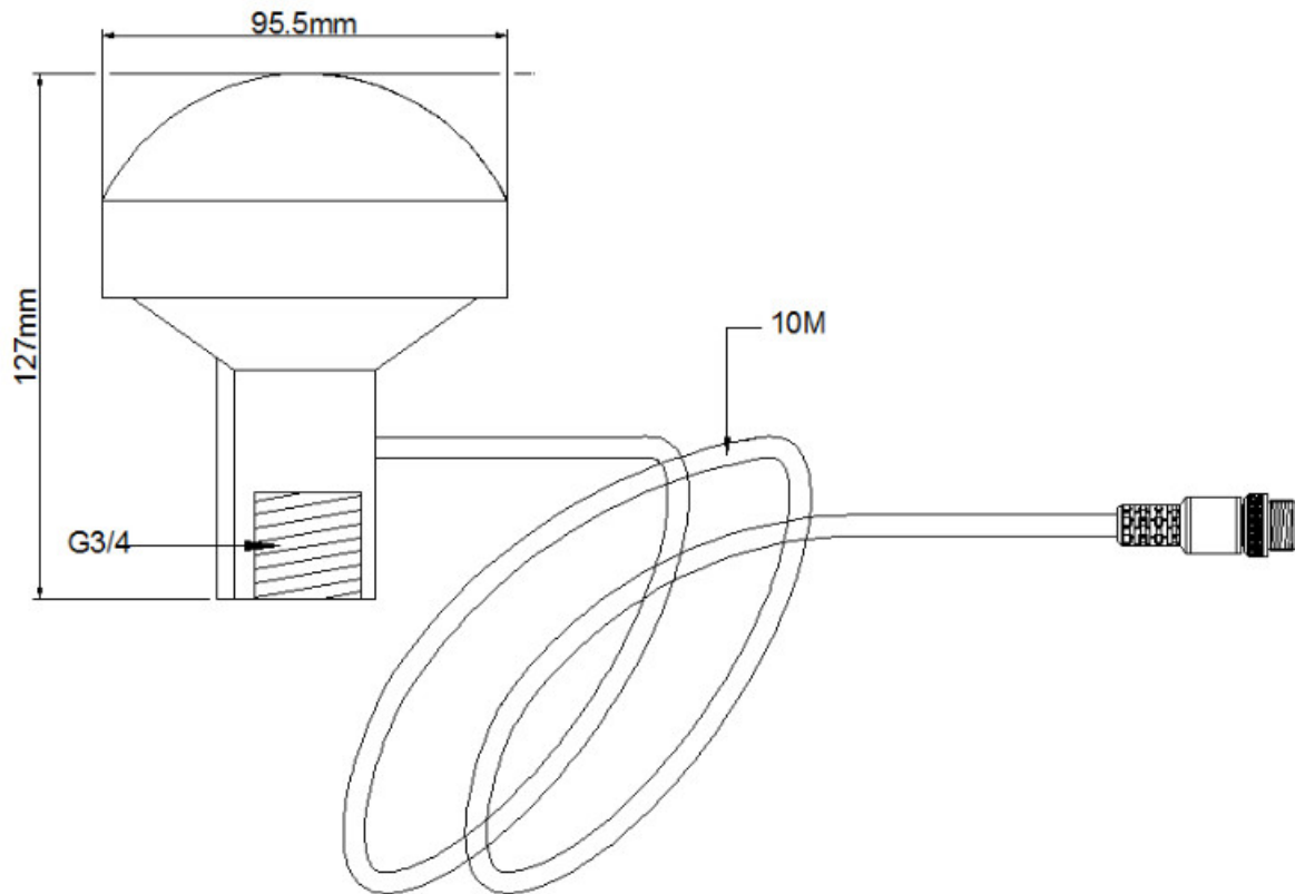
Figure 1 AS07-N2K Dimensions
