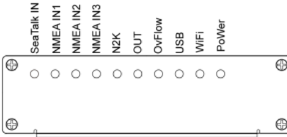
Figure 2: LED indications
