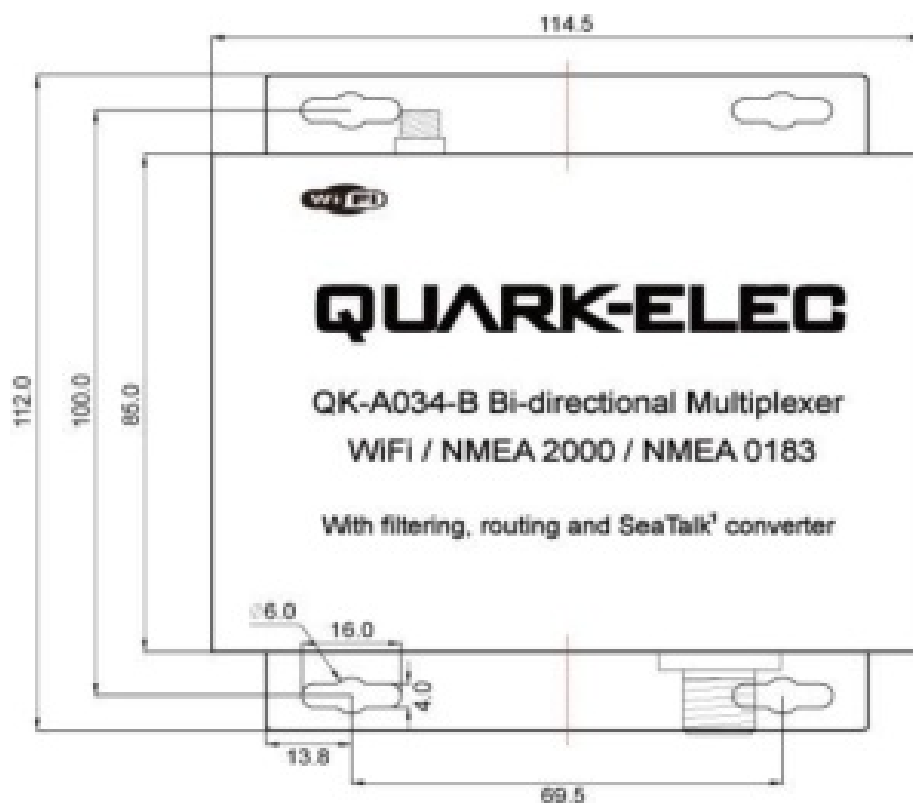
Figure 1 Dimensions
