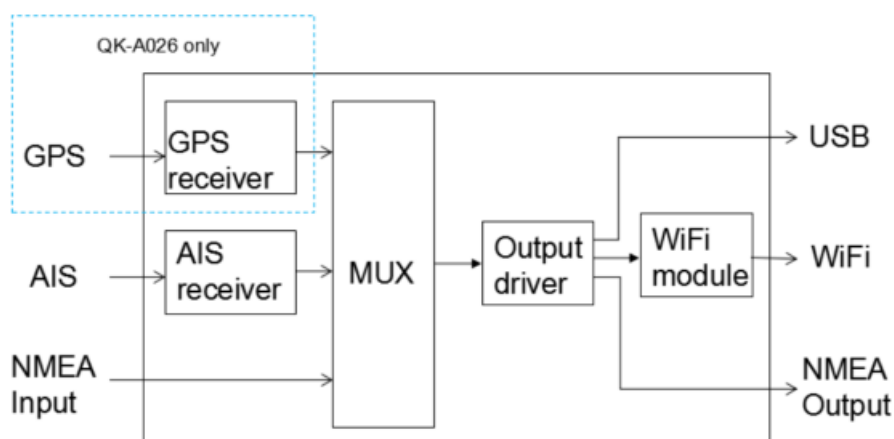
Figure 1: A024/26 Function diagram
