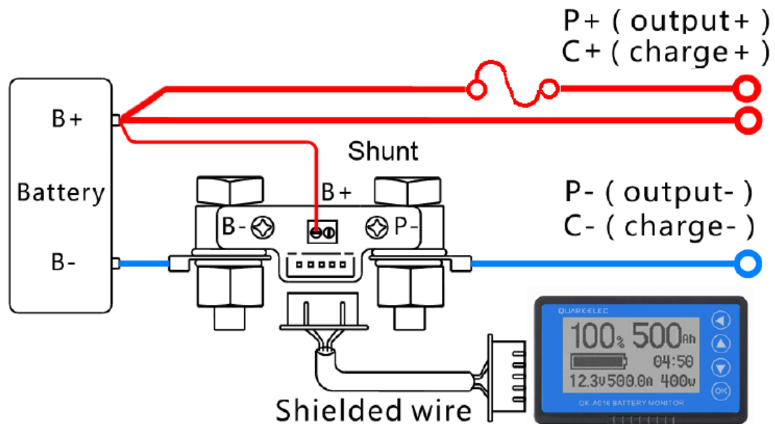
Figure 1 A016 wiring diagram
