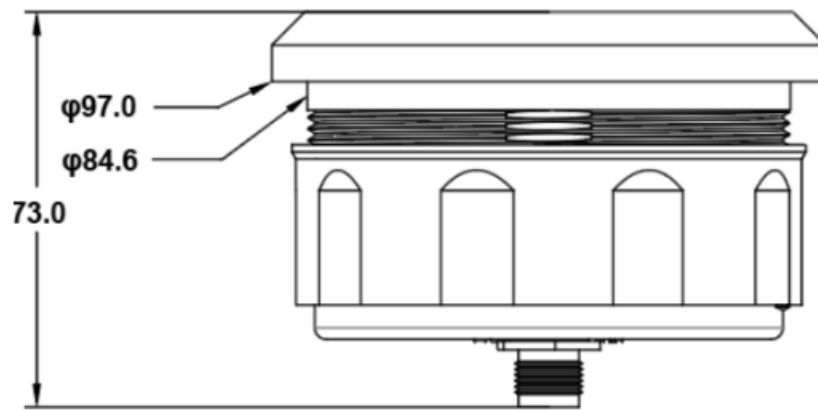
Figure 2: Dimensions(mm) for Flush Mounting
