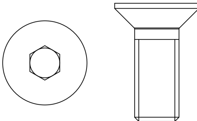
Screw M3x8 DIN7991 (2 pcs)
