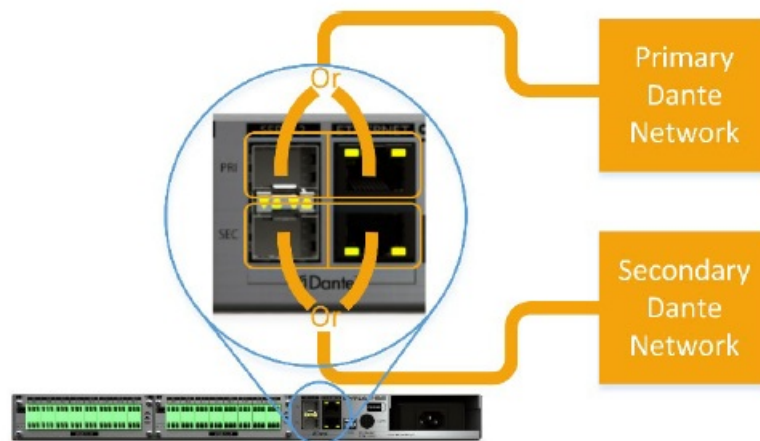
Figure 4 – “Redundant” mode, no daisy chain
