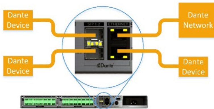
Figure 7 - "Standalone" connection in "Switched" mode
