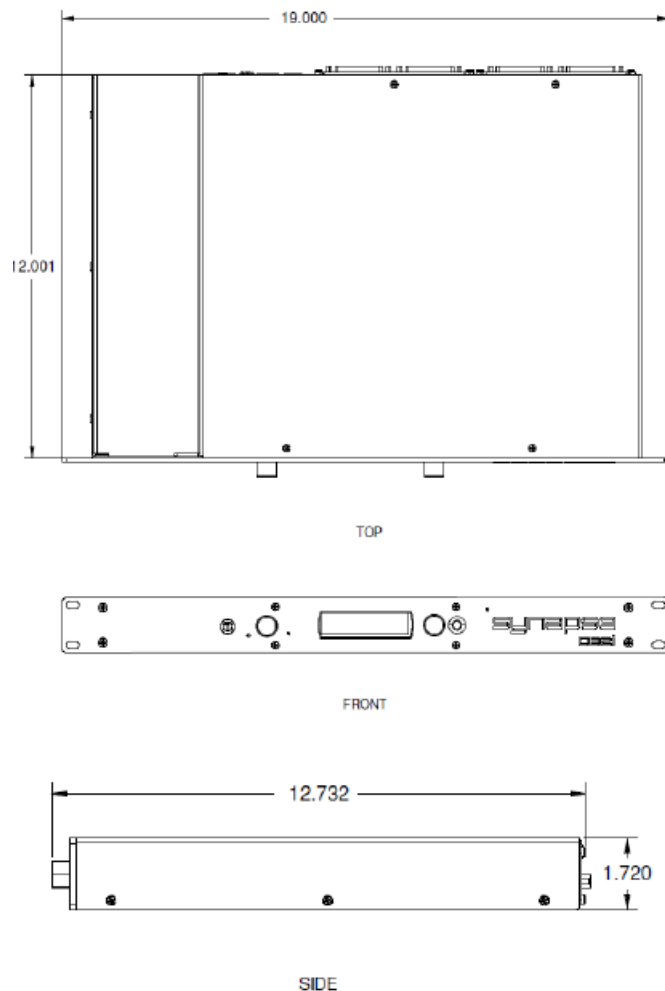
Figure 1 - Mounting and Dimension Information
