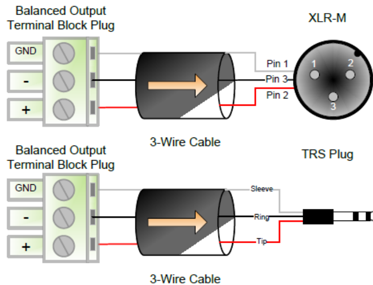
Figure 2 - Balanced Wiring Guide
