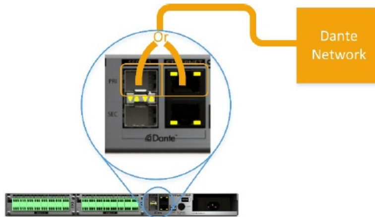
Figure 6 - "Standalone" connection in "Redundant" mode
