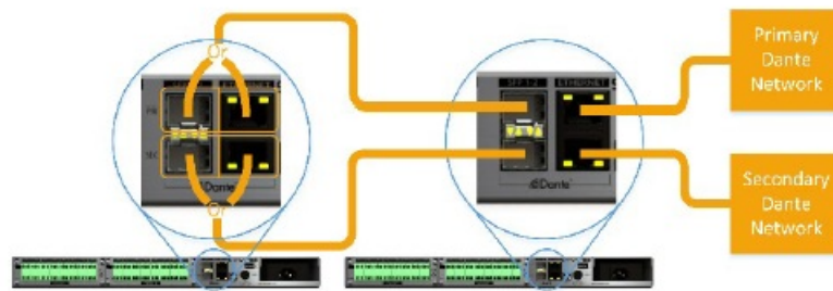
Figure 5 - "Redundant" mode with daisy chaining
