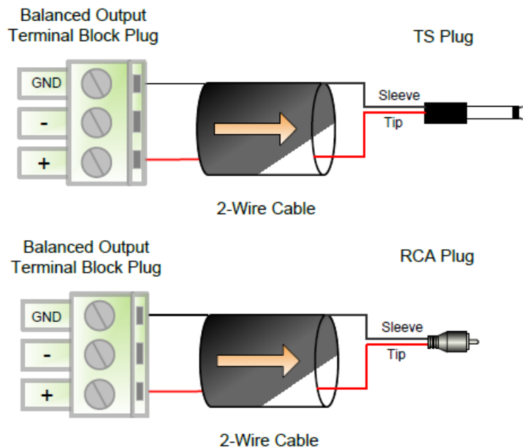
Figure 3 - Unbalanced Wiring Guide
