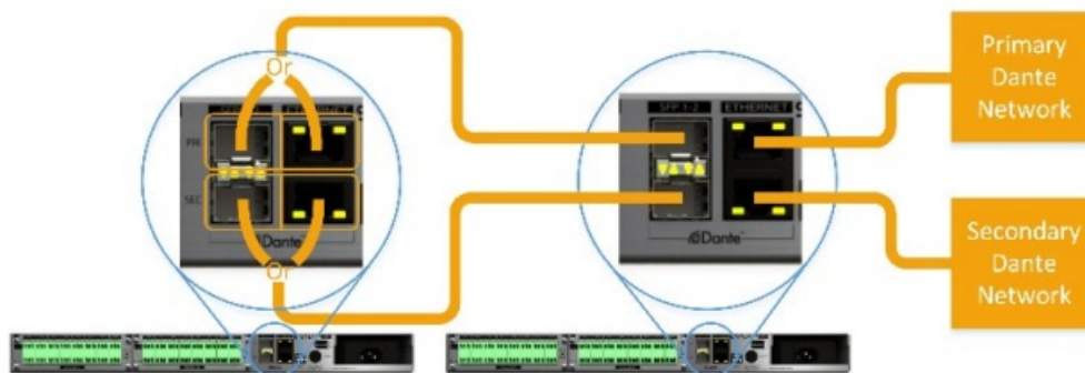
Figure 5 - "Redundant" mode with daisy chaining
