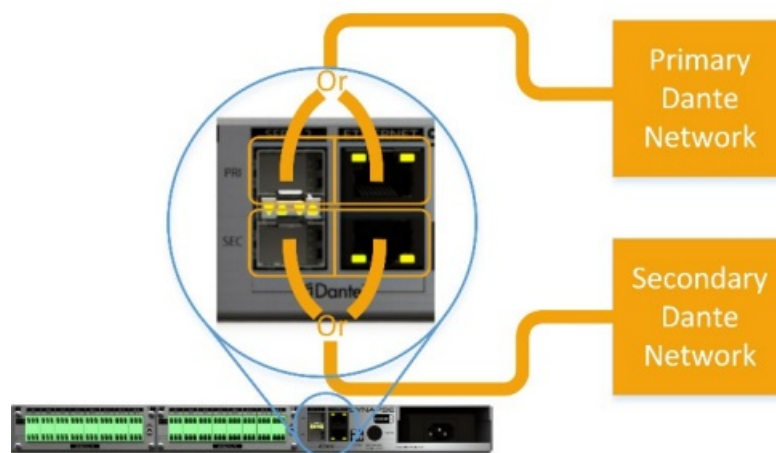
Figure 4 – “Redundant” mode, no daisy chain
