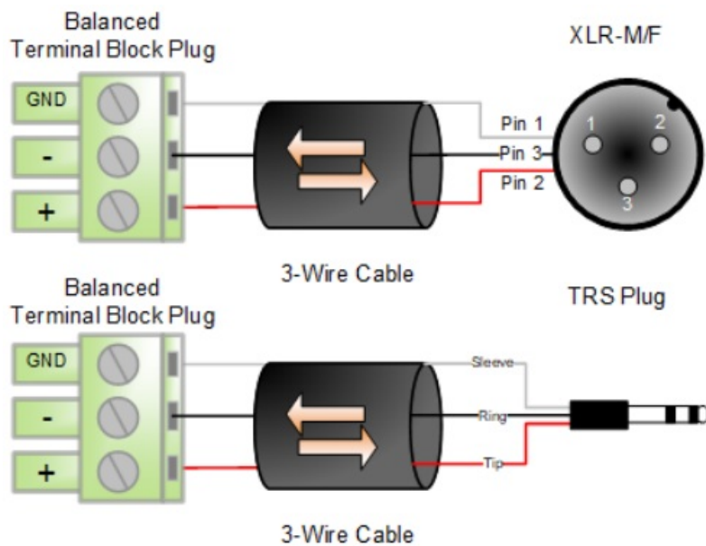
Figure 2 - Balanced Wiring Guide
