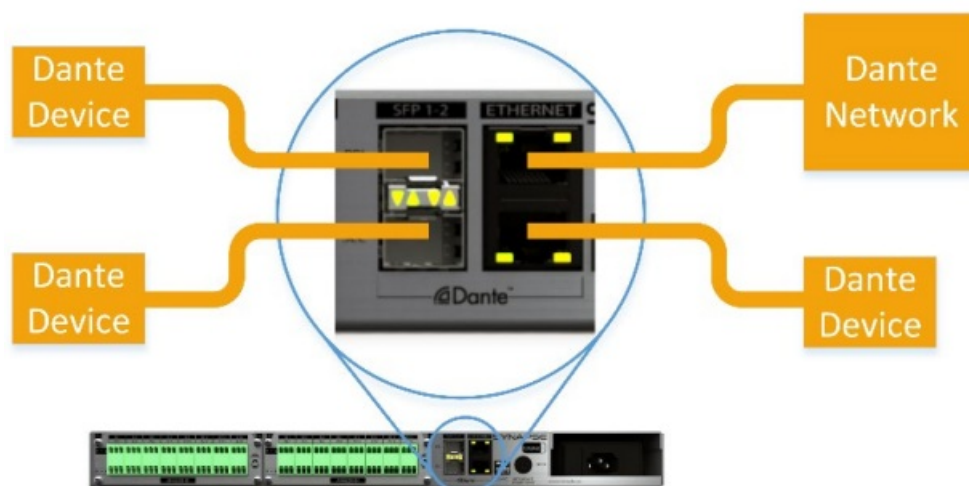
Figure 7 - "Standalone" connection in "Switched" mode
