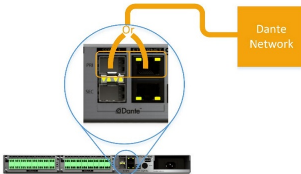
Figure 6 - "Standalone" connection in "Redundant" mode
