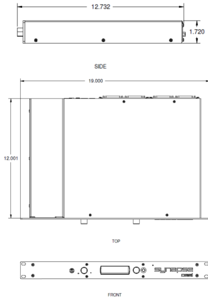
Figure 1 - Mounting and Dimension Information
