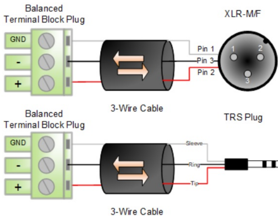
Figure 2 - Balanced Wiring Guide
