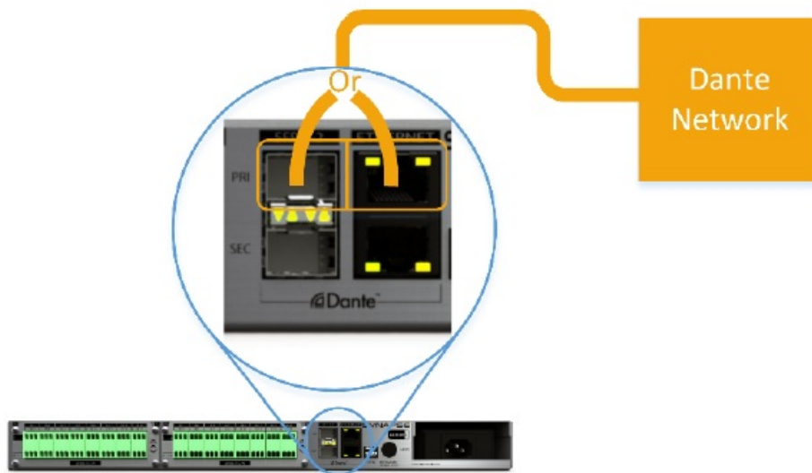
Figure 6 - "Standalone" connection in "Redundant" mode
