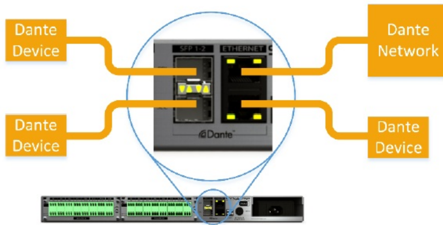
Figure 7 - "Standalone" connection in "Switched" mode
