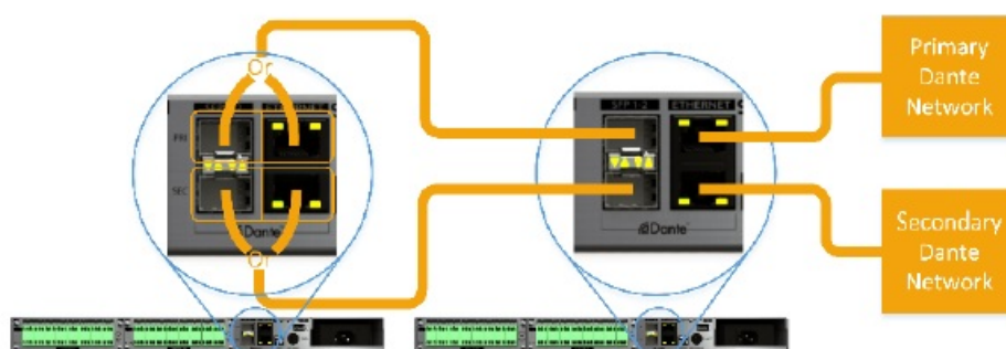
Figure 5 - "Redundant" mode with daisy chaining
