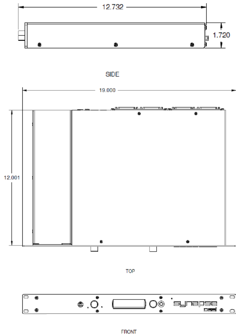
Figure 1 - Mounting and Dimension Information
