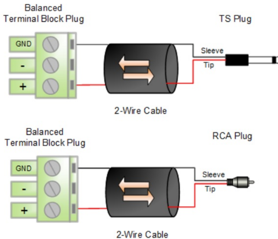
Figure 3 - Unbalanced Wiring Guide
