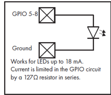
Q-SYS-Powered LED
