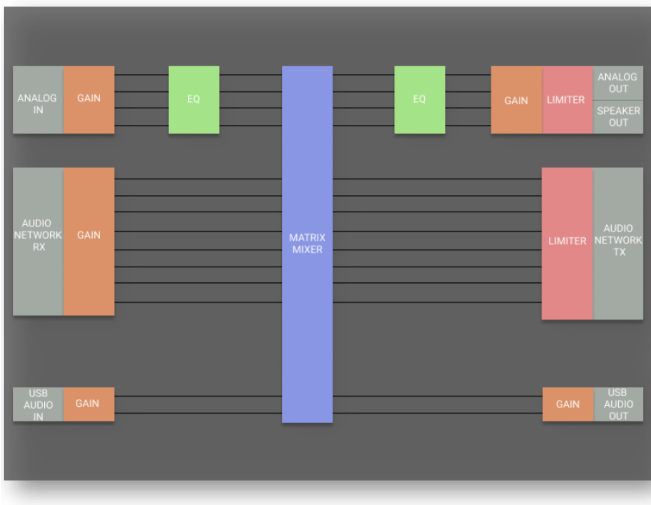
11 - DSP Signal Flow Diagram
