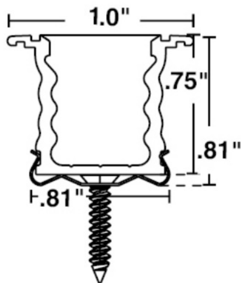
Profile with stainless steel mounting clip
