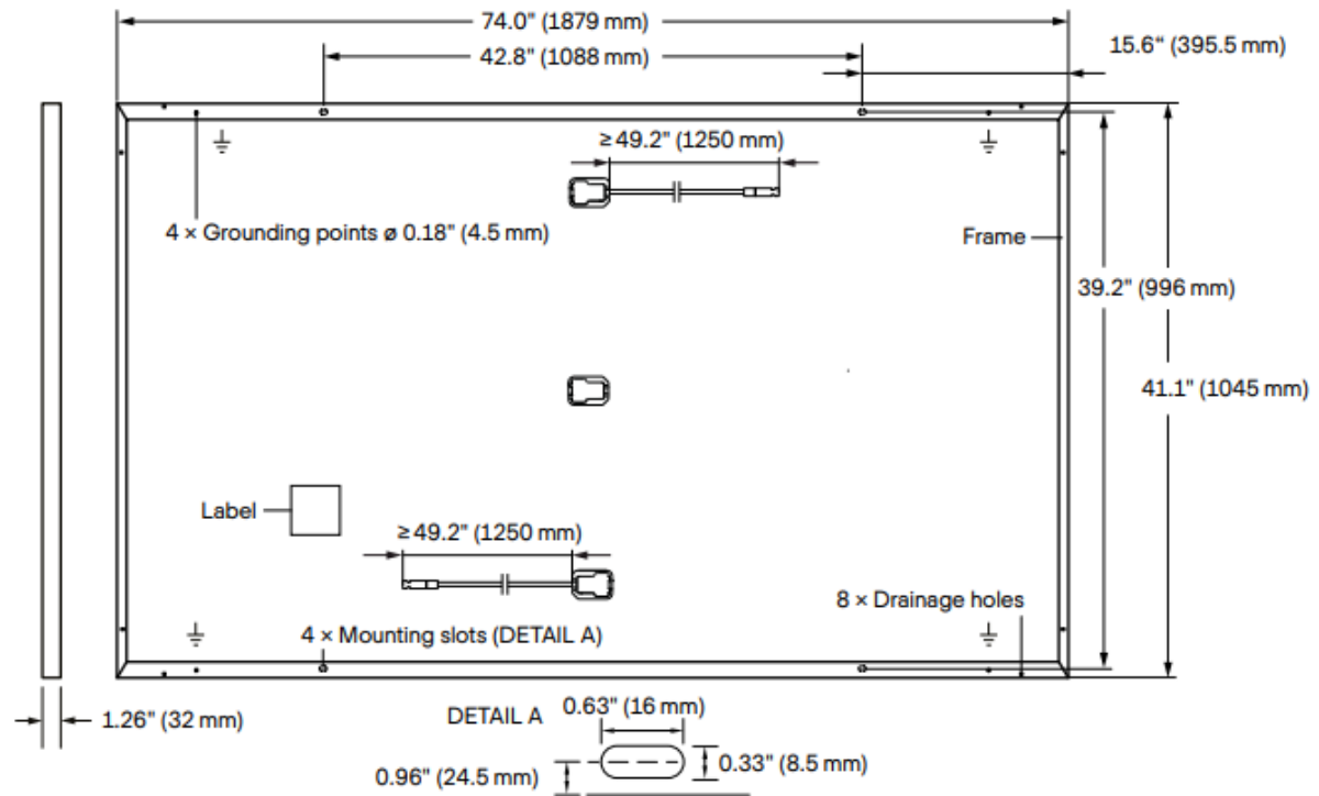
Fig. 1: External dimensions (in inch (mm)) and components for
