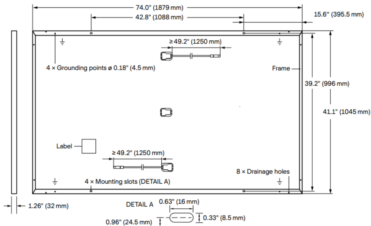
Fig. 2: External dimensions (in inch (mm)) and components for
