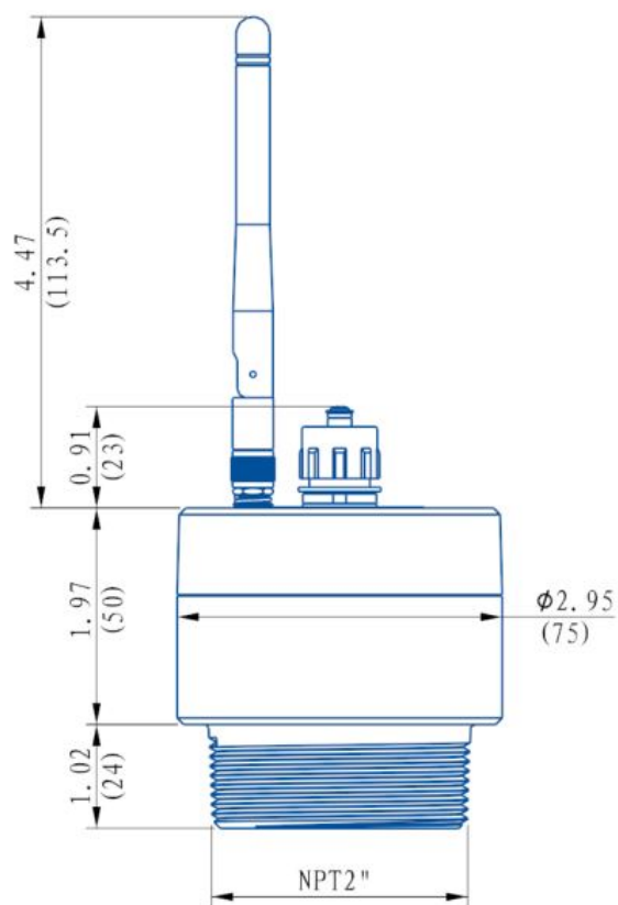
LSR-801L Dimension
