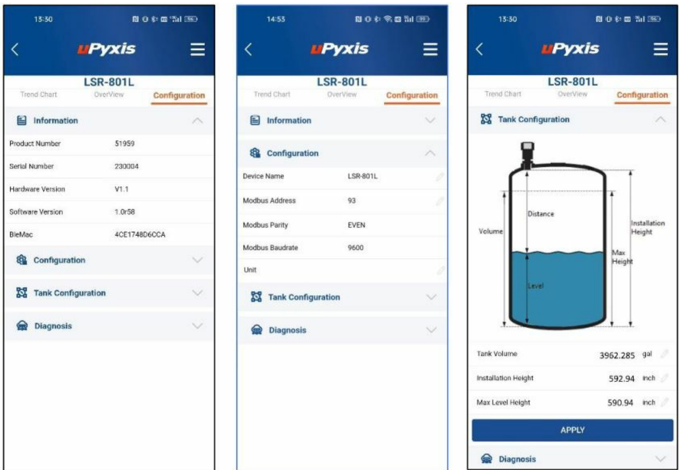
Figure 6. Sensor Configuration
