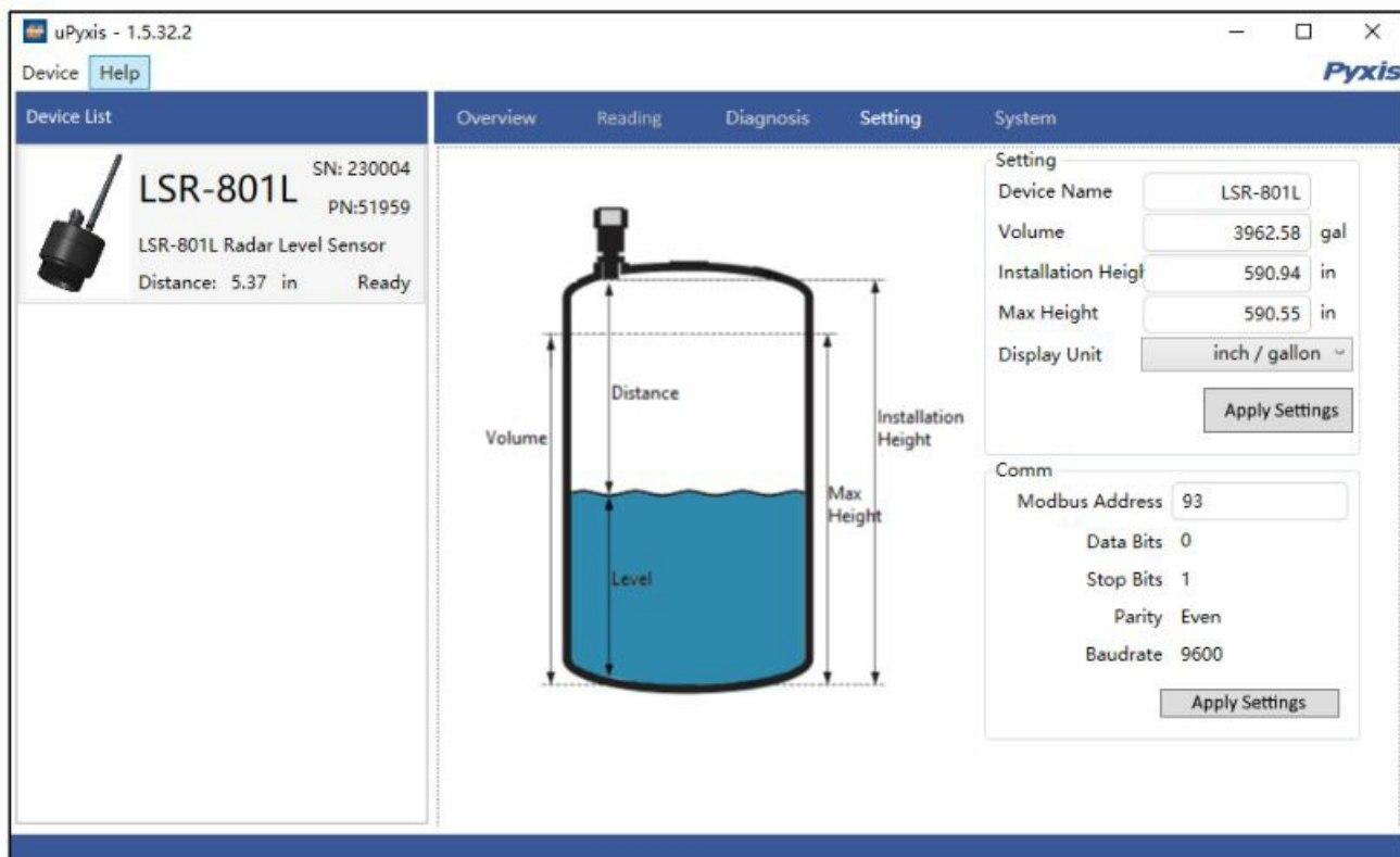
Figure 10. Illustration of terms and tank capacity setup
