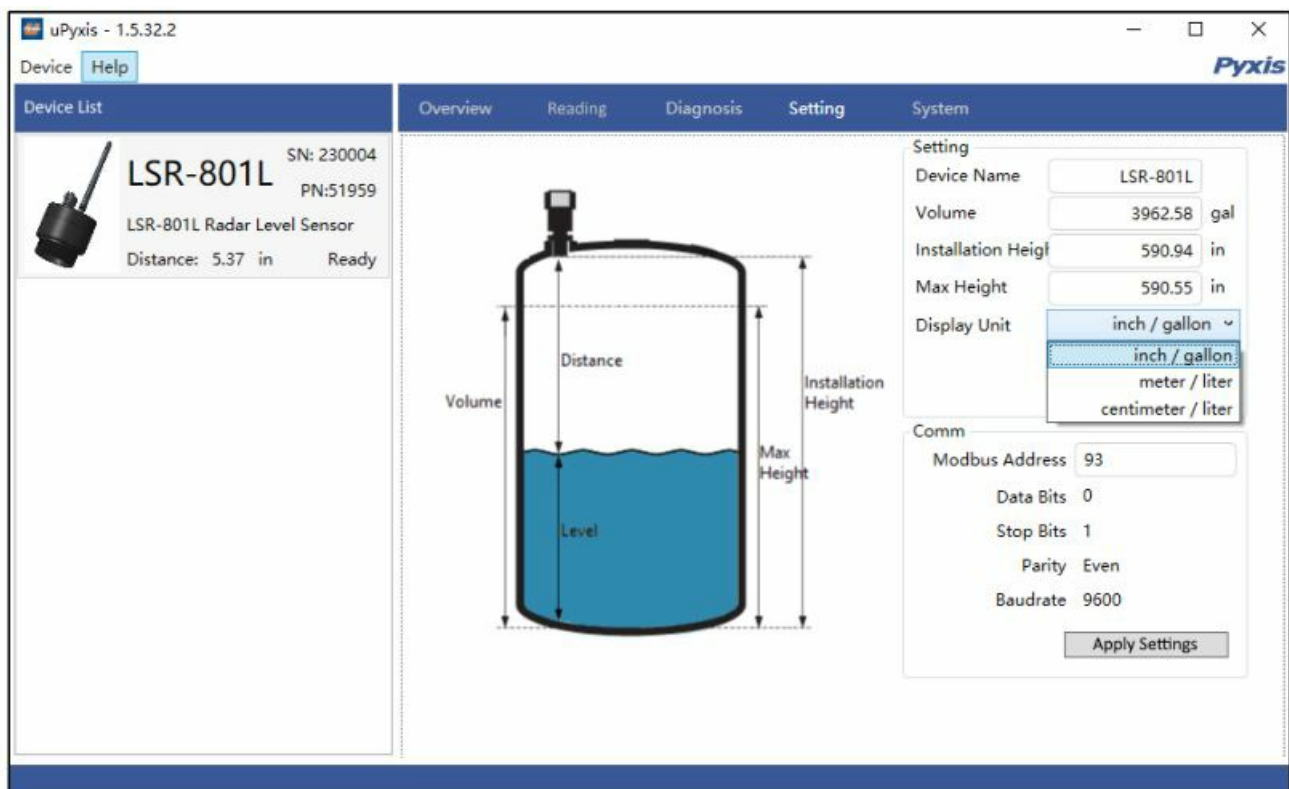
Figure 11. Display Unit Dropdown Selection
