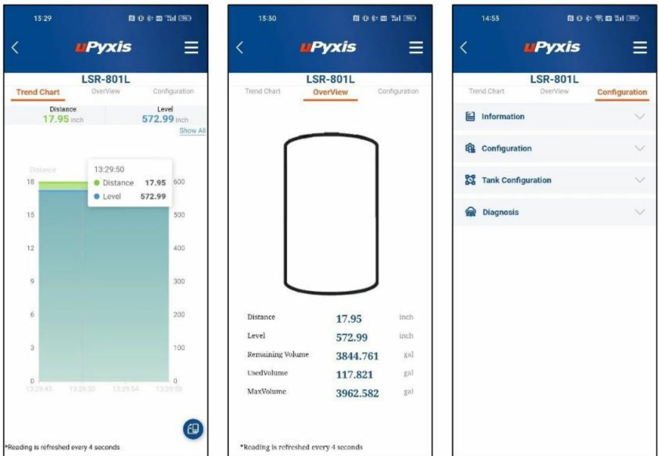
Figure 5. Sensor Tab Selection
