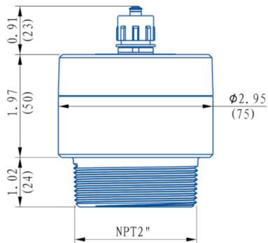
LSR-801 Dimension
