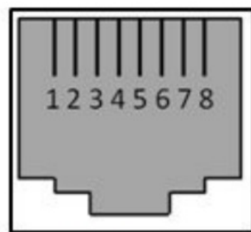
RJ45 Port
