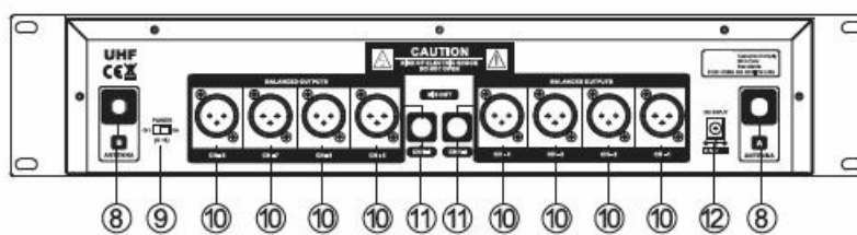
Rear Panel
