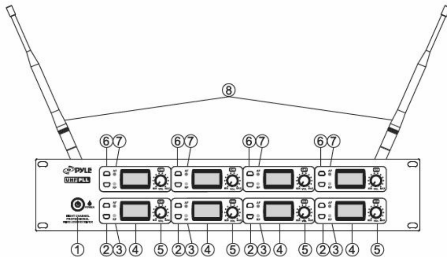
Front Panel
