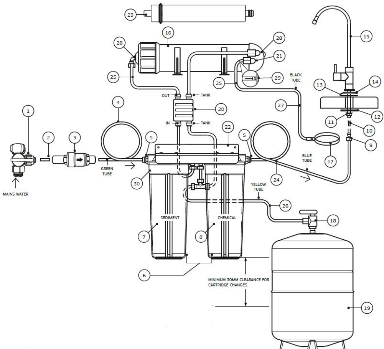
Figure 1 – Parts Diagram
