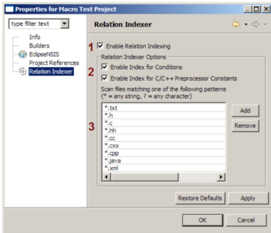
Figure 5. Project Property Page for the Relation Indexer
