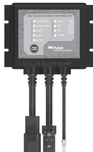
Figure 2: PT20 Top View
