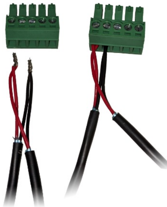
RS-485 Home-Run connection
