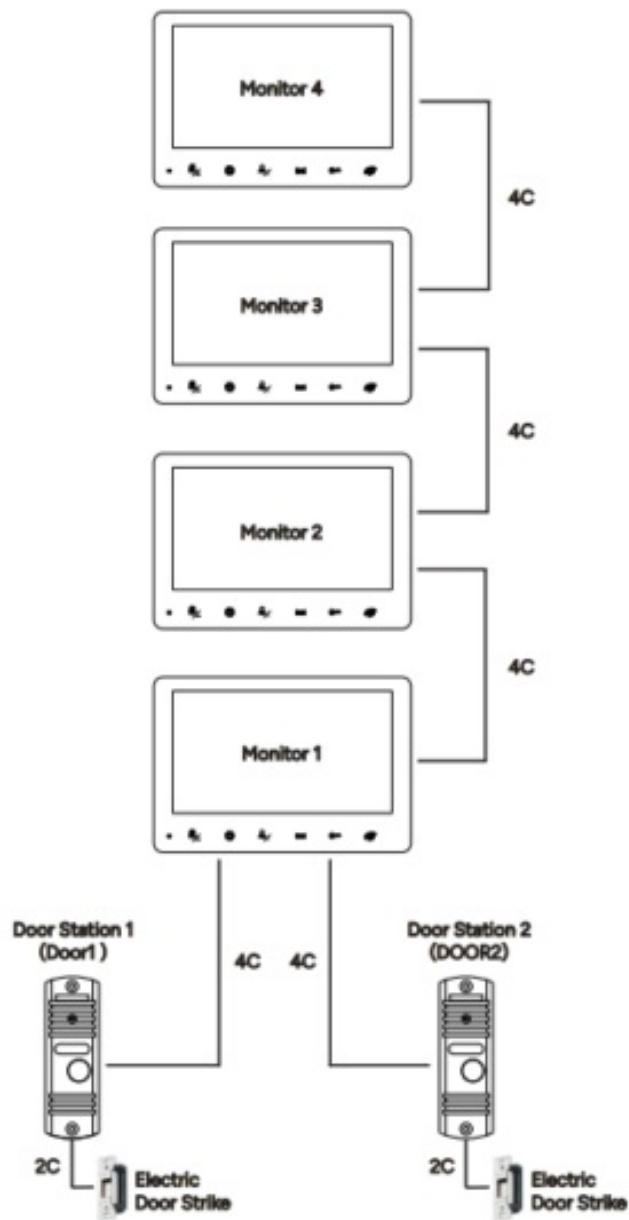
System Wiring Diagram
