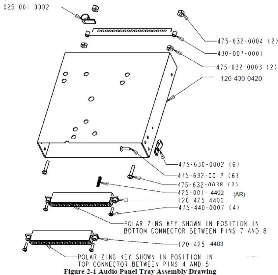
Figure 2-1 Audio Panel Tray Assembly Drawing
