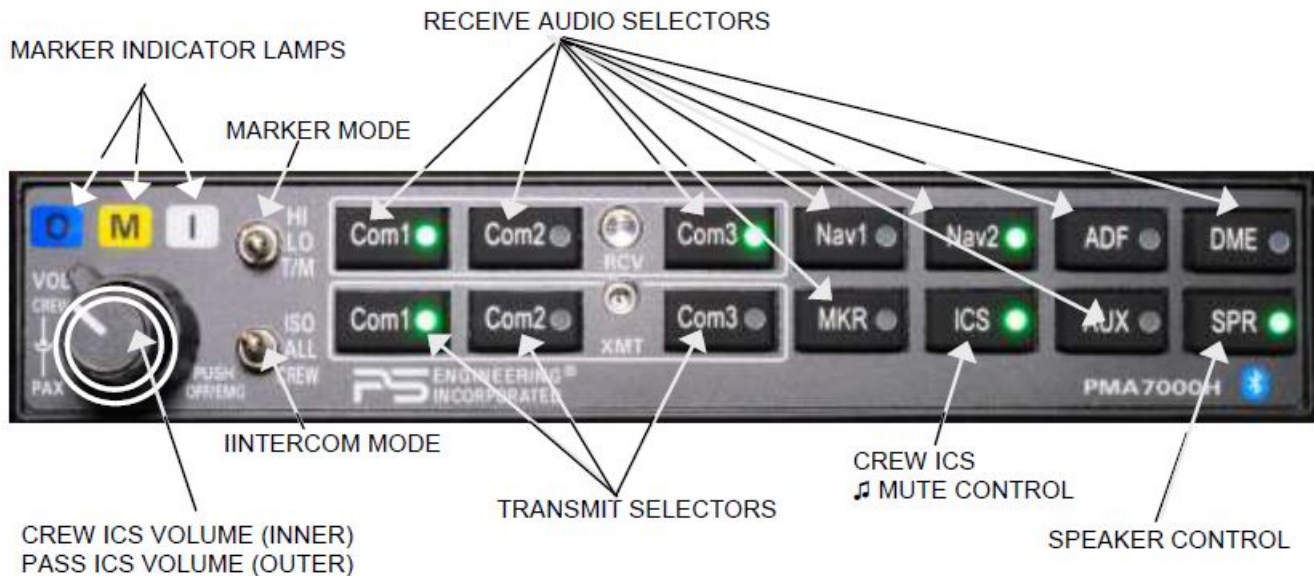
Figure 3-1 PMA7000H-BT controls
