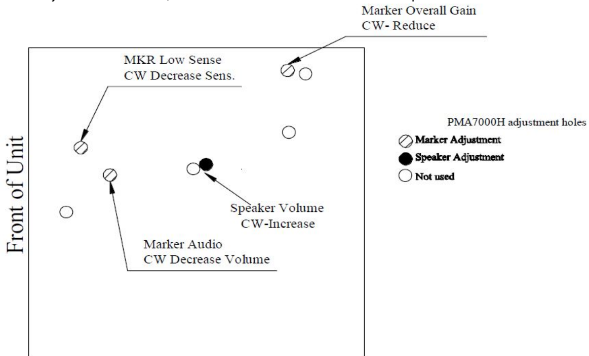
Figure 2-3- PMA7000H-BT Adjustments
