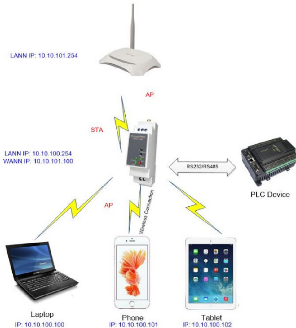
Figure 8. AP+STA Wireless Network
