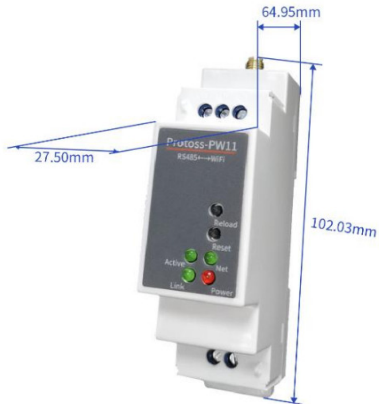
Figure 3. Protoss-PW11 Mechanical Dimension
