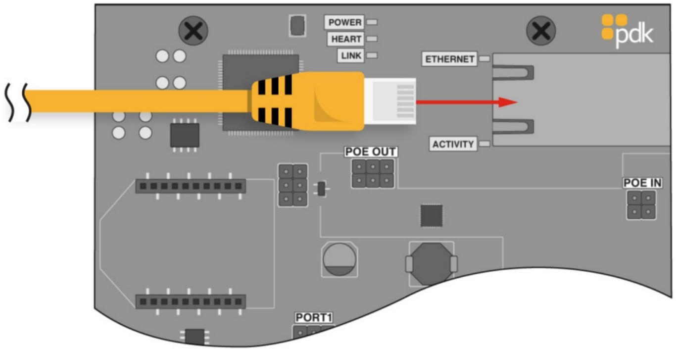
Standard Ethernet Board – An Ethernet connection is one of the Red Gate communications option.
