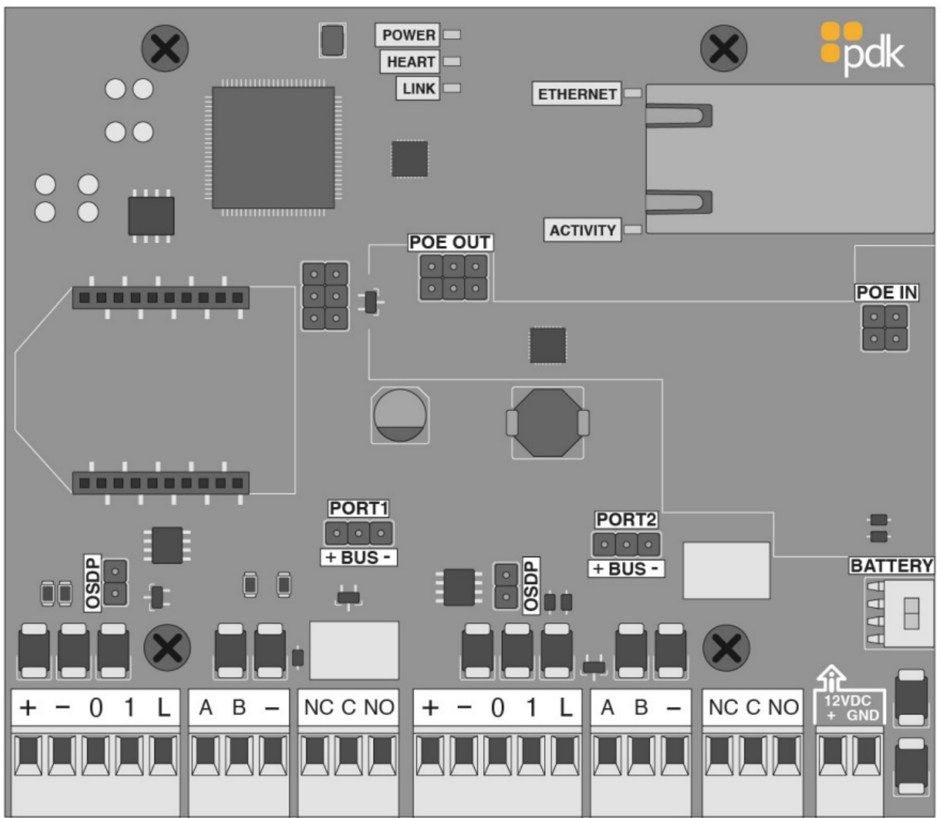
Standard Ethernet Board – An Ethernet connection is one of the Red Gate communications option.
