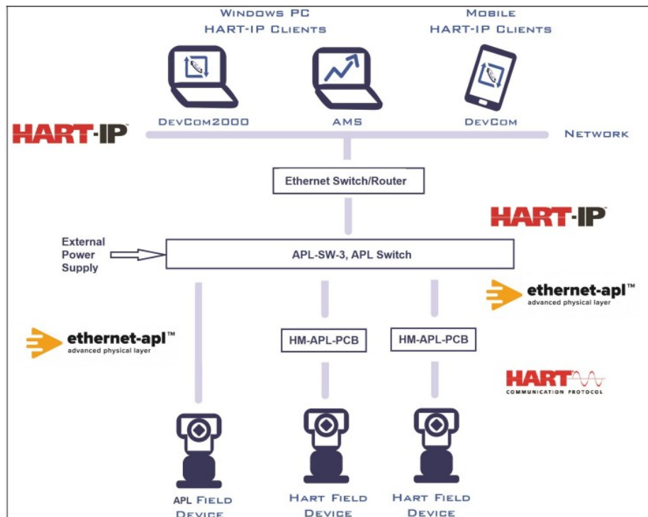
Figure 1. APL-SW-3 System Diagram
