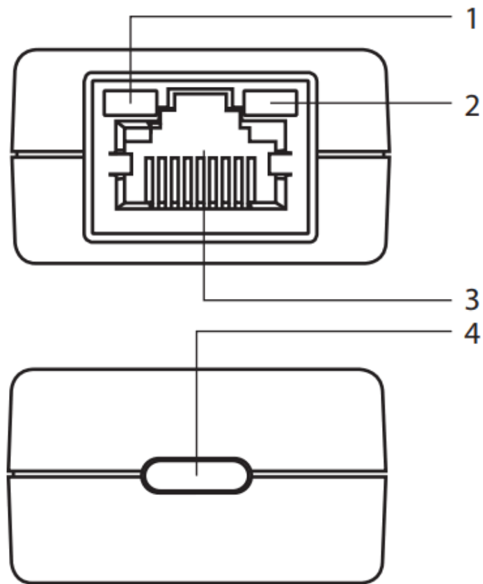
2-1 Product Working Diagram
