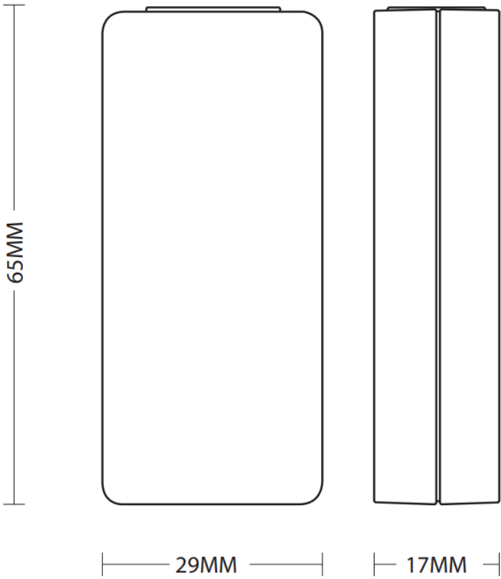
Pic3-1 Product Dimensions
