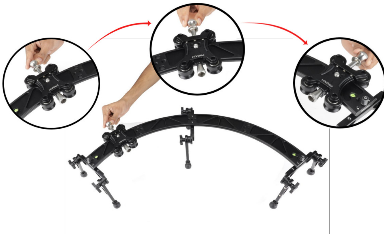
Proaim Curve-120 curved camera slider with Motion Control System.
