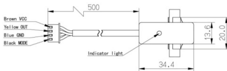
Y26A wiring diagram of various models
