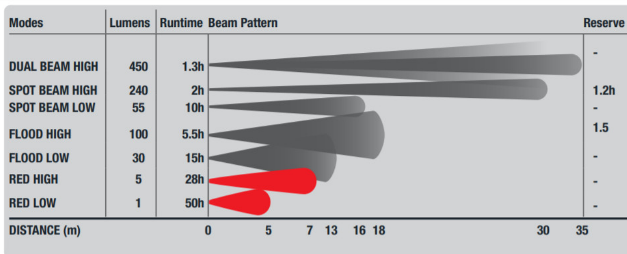
Figure 3 – Performance
