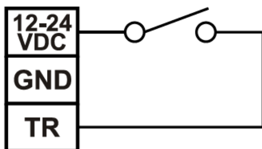
Positive Trigger (Dip switch B1 OFF)
