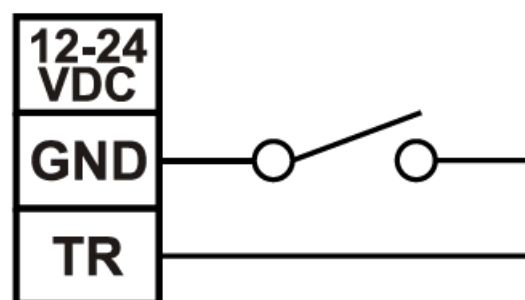
Negative Trigger (Dip switch B1 ON)
