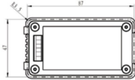
Figure 16 Hole size
