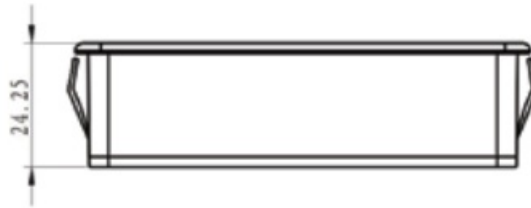
Figure 17 Height size
