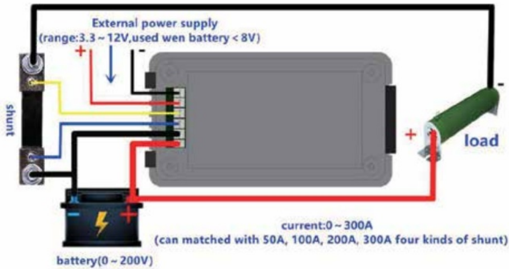
Figure 13 Wiring Diagram
