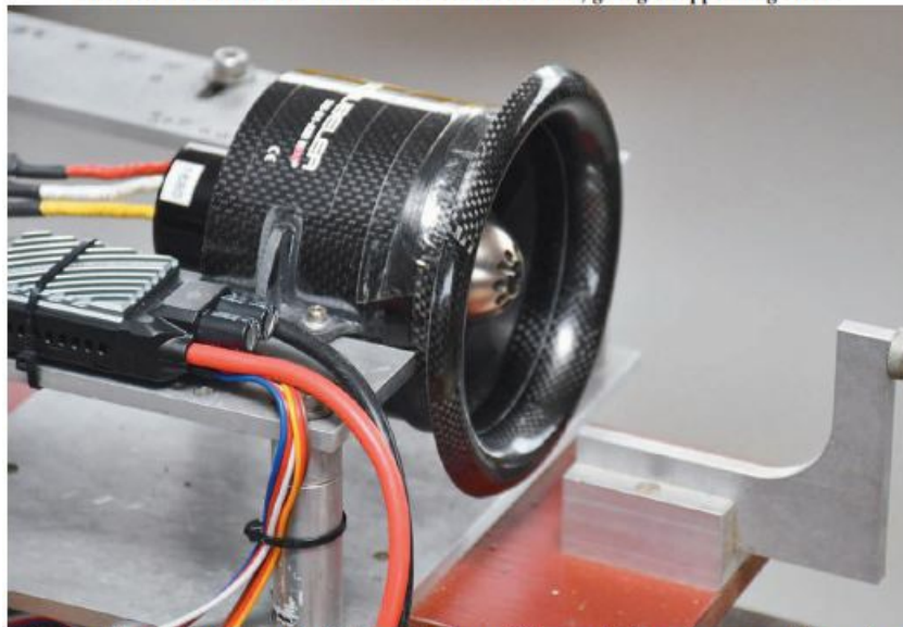
Testing with the intake moulding fitted made a huge difference to the performance of the system
