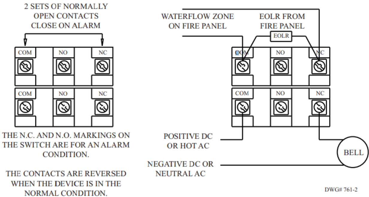
FIG. 3 TYPICAL ELECTRICAL CONNECTIONS
