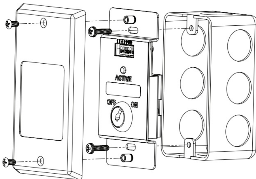
PAD100-LEDK Back View and Wiring
