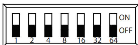
FIGURE 9: Enlarged View of PAD Device with Dip Switch Setting Unaddressed
