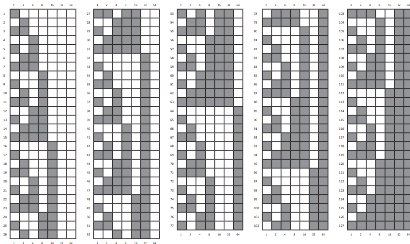
NOTE: Each gray box indicates that the dip switch is ON and each white box indicates the dip switch is OFF. FIGURE 11: PAD Device Dip Switch Addresses Table (Addresses 1-127)
