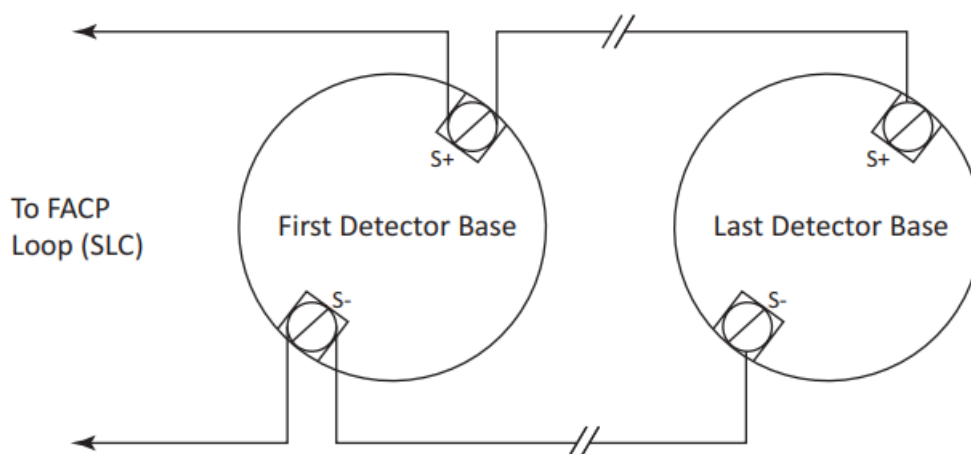
Figure 1 Wiring (Style B) Using PAD100-6DB or PAD100-4DB
