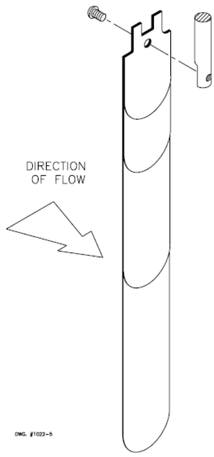
Fig. 3 Typical paddle arrangement for 6" to 8" pipe.
