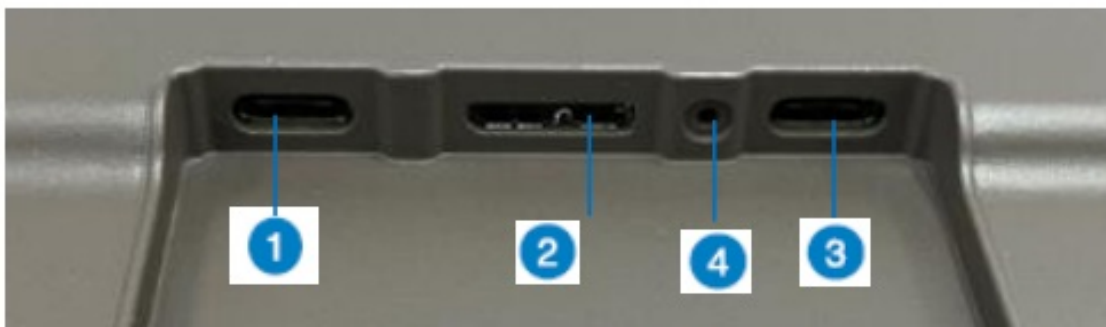
Figure 1-3: MICROS Workstation 8 I/O View
