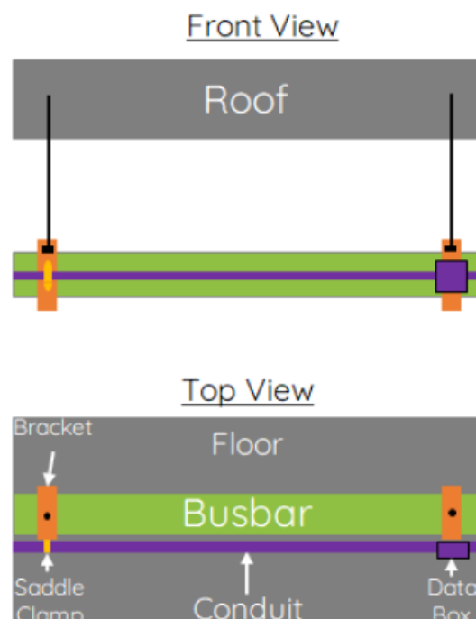
Figure 16. Roof Suspended (not to scale)
