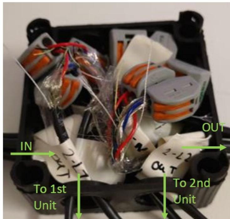
Figure 36. Data Box with two Chargepoints connected
