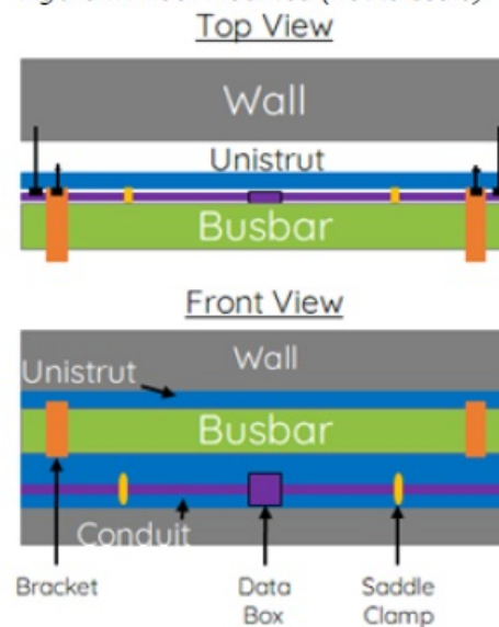
Figure 18. Wall Mounted (not to scale)
