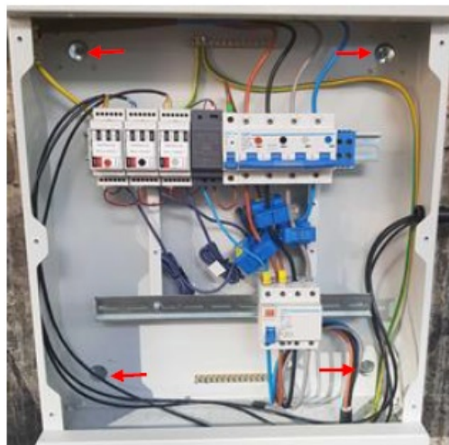
Figure 2. Distribution Board fixing locations
