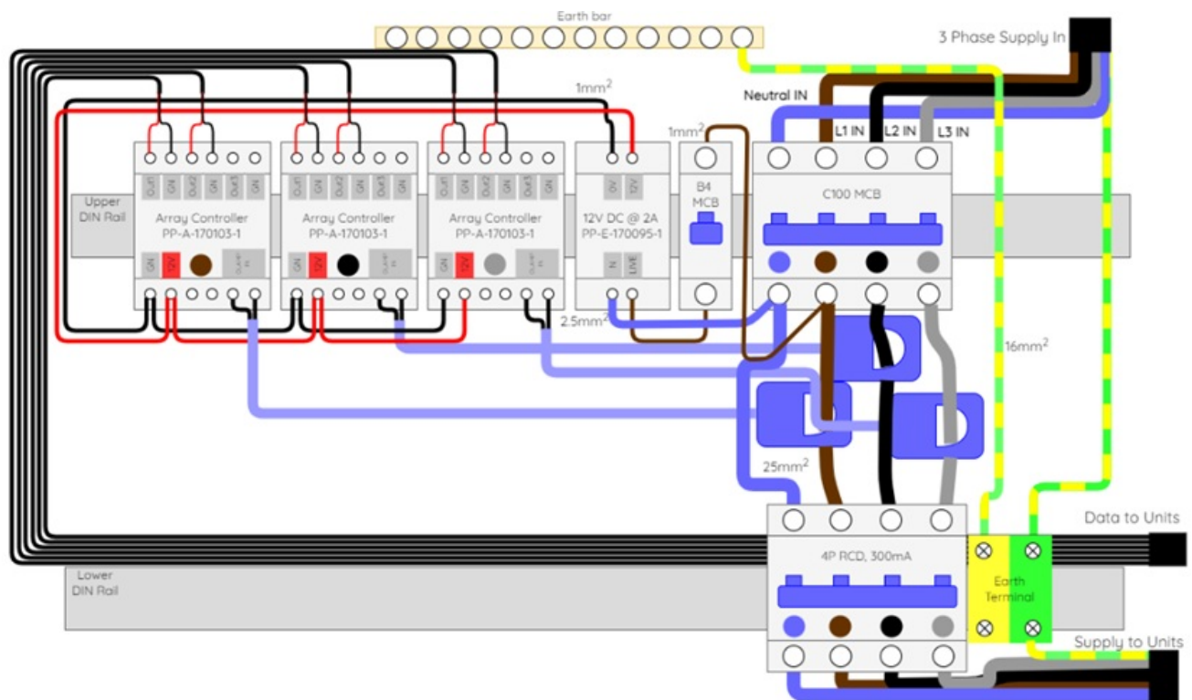
Figure 8. Distribution Board diagram of AC-DB-01-UAA -One-way busbar
