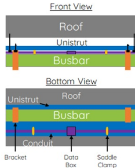
Figure 17. Roof Mounted (not to scale)
