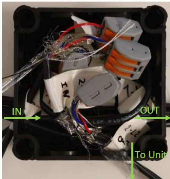
Figure 35. Data Box with one Chargepoint connected
