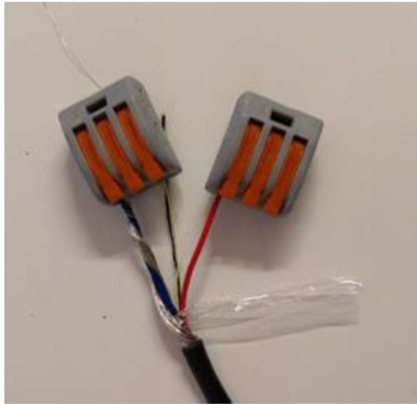
Figure 30. Incoming Data cables as if fitted to a unit, only showing 1 phase pair of Data Cables for clarity
