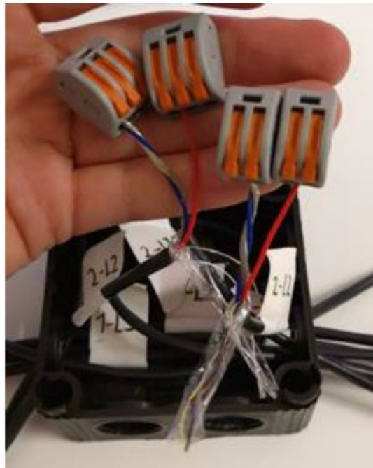
Figure 32. Incoming and outgoing Data cables wired into 3 and 2 lever terminals
