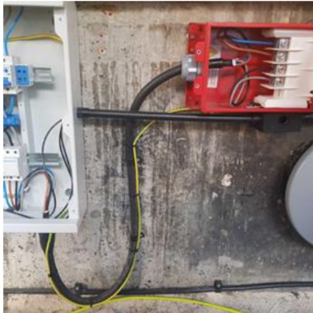
Figure 3. Example set-up for connecting Distribution Board to Feeder Unit
