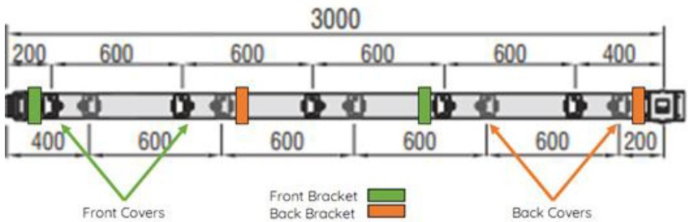
Figure 15. Idealised Bracket Spacing on example 3m length
