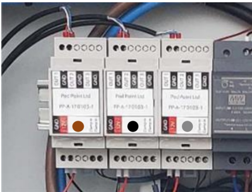
Figure 11. Array Controller connections – showing only 1x per phase for simplicity Feed Data cables through conduit(s) to the first Data Box, attached to the first bracket.
