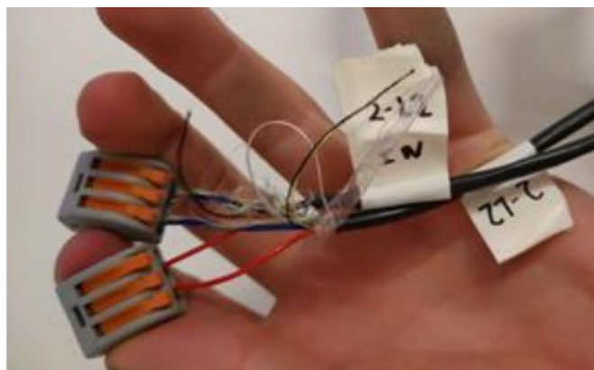
Figure 33. Data cable to the Chargepoint fitted to the 3-lever terminals
