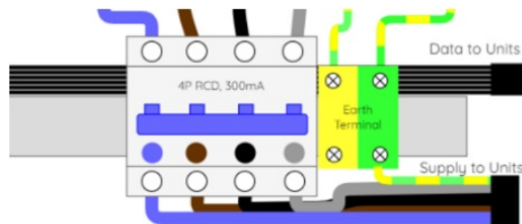
Figure 9 Supply to Busbar for AC-DB-01-UAA - One-way
