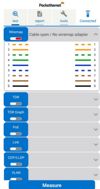
Open cable
