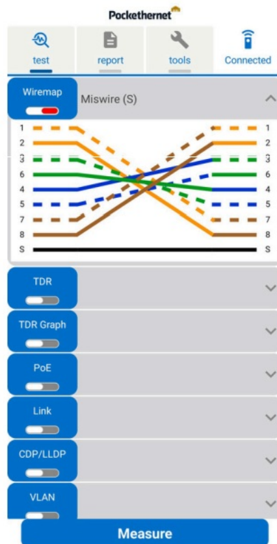
Miswired cable
