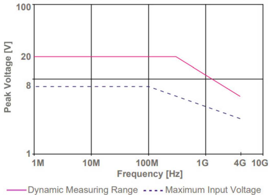
Input Voltage - HSDP2010 / HSDP2010L / HSDP4010
