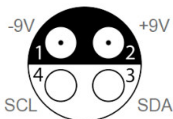
Probe's power supply pin assignment "cable view"
