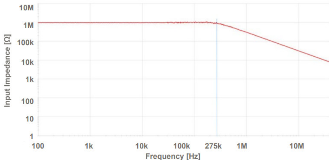
Typical Differential Input Impedance - HSDP Series
