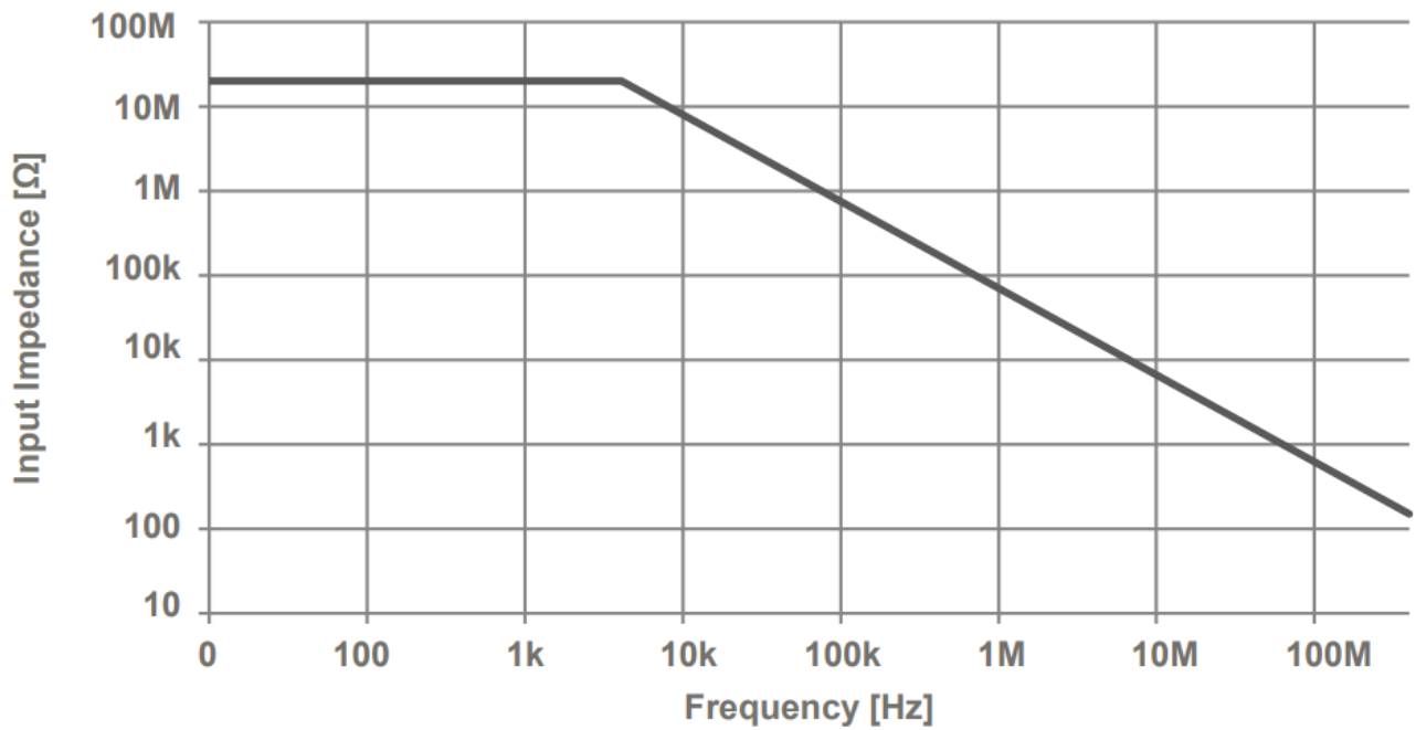
Typical Differential Input Impedance – HORNET4kV
