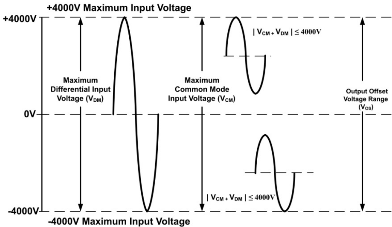
Maximum Input Voltage, Example 4000V Model, 100:1 Range
