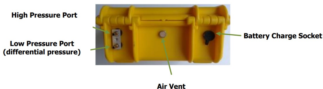
Figure 9 - CONNECTING TUBES
