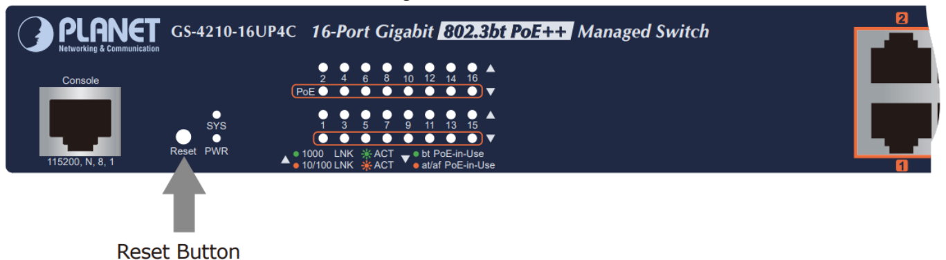
Figure 5-2: GS-4210-16UP4C Reset Button
