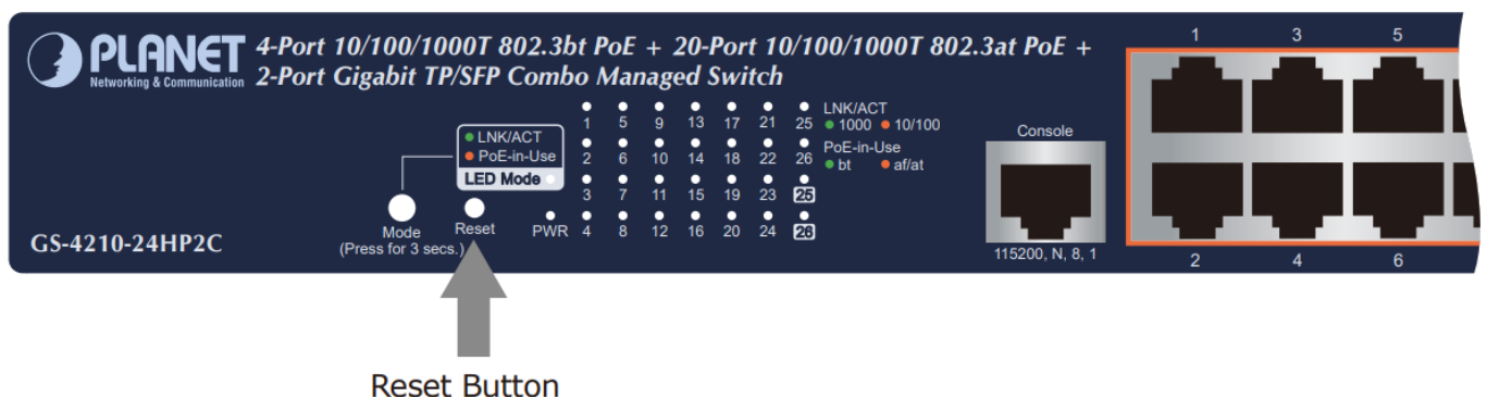
Figure 5-4: GS-4210-24HP2C Reset Button
