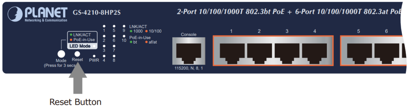
Figure 5-1: GS-4210-8HP2S Reset Button
