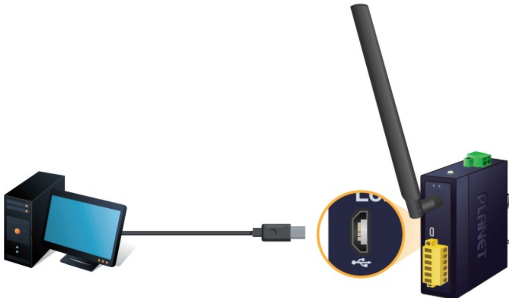
Figure 6: Connecting LoRa Node Controller to computer via Micro USB Cable
