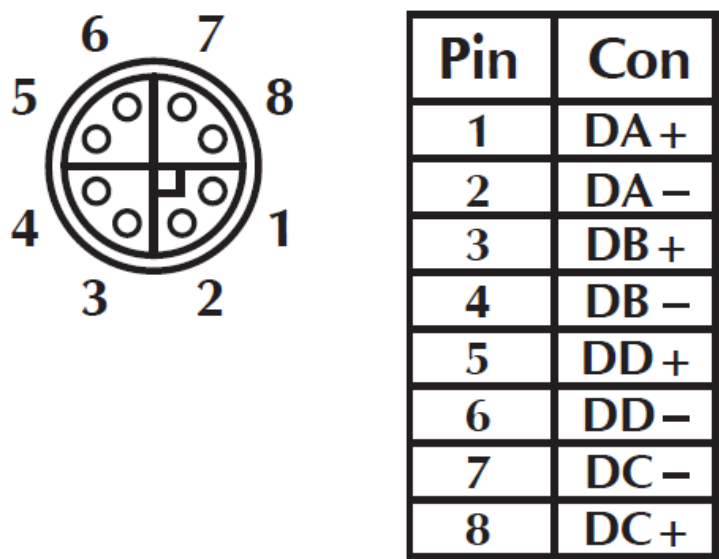
8-pin M12 X-coded Female 10/100/1000T Connector Pin Assignment
