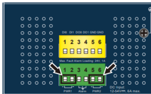
Figure 3-2: IGS-5225-8P4S-12V Upper Panel
