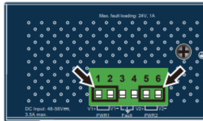
Figure 3-4: IGS-5225-4P2S Upper Panel
