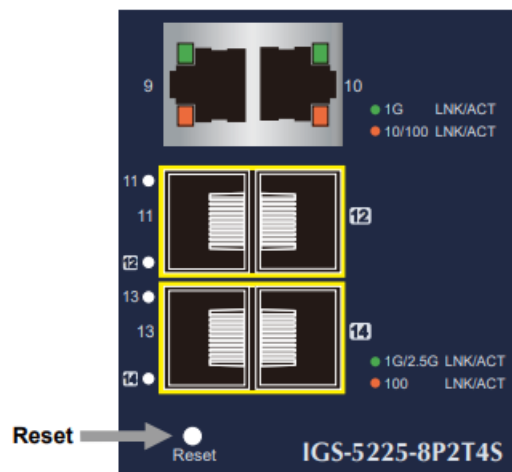
Figure 6-4: IGS-5225-8P4S/IGS-5225-8P4S-12V/IGS-5225-8P2T2S/ IGS-5225-8P2T4S Reset Button
