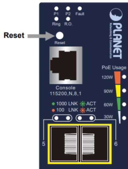
Figure 6-2: IGS-5225-4P2S Reset Button
