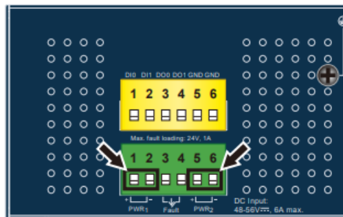
Figure 3-5: IGS-5225-4UP1T2S Upper Panel
