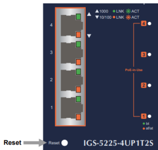
Figure 6-3: IGS-5225-4UP1T2S Reset Button
