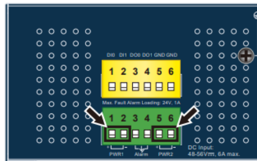
Figure 3-1: IGS-5225-8P4S/IGS-5225-8P2T2S/IGS-5225-8P2T4S Upper Panel
